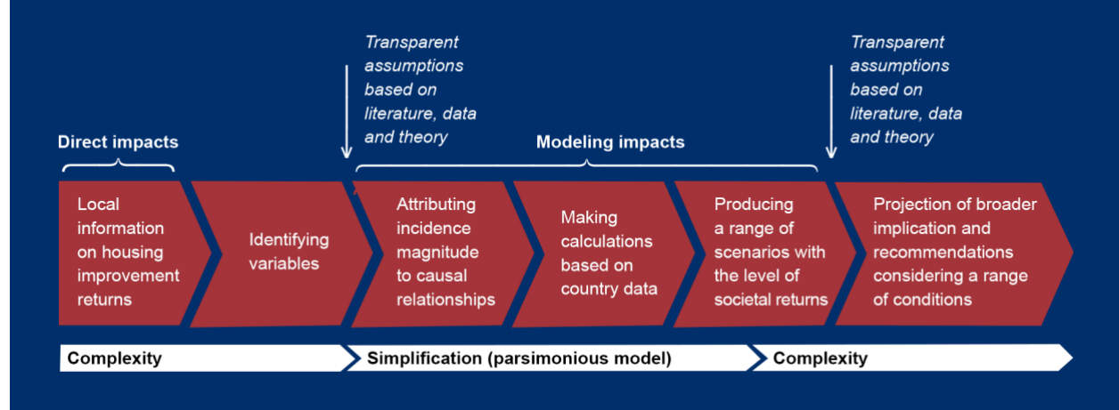
Figure 2: Methodological approach
